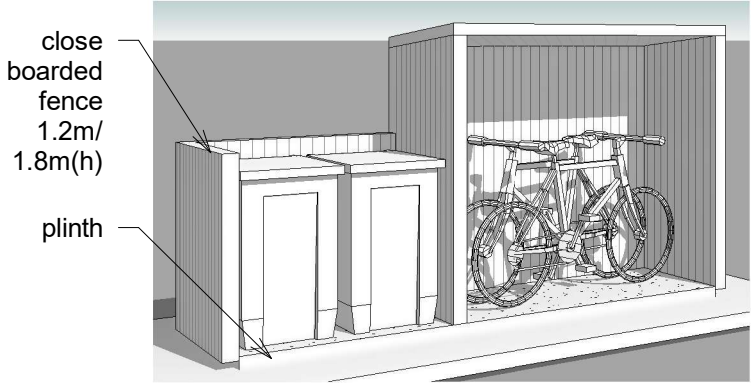
3 Typ. Bin and Cycle Store (3D)
