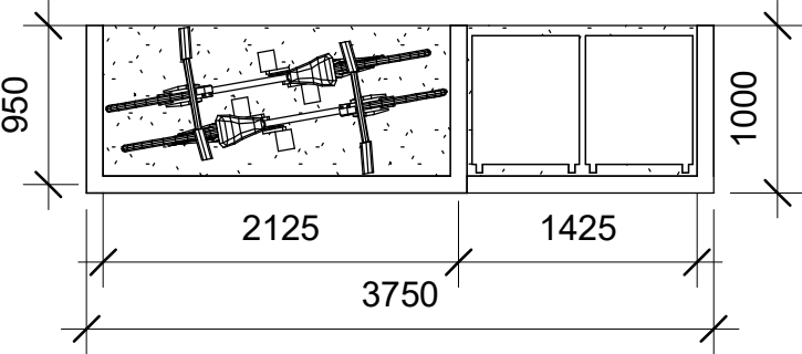
2 Typ. Bin and Cycle Store 1 : 50
