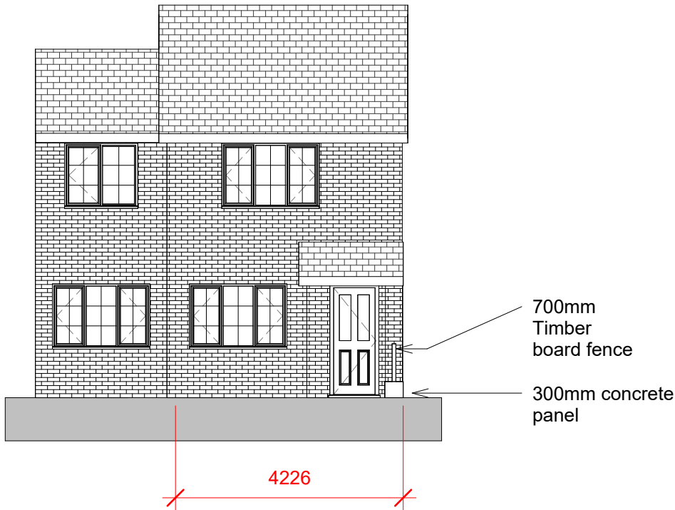
Front Elevation 1 : 100
