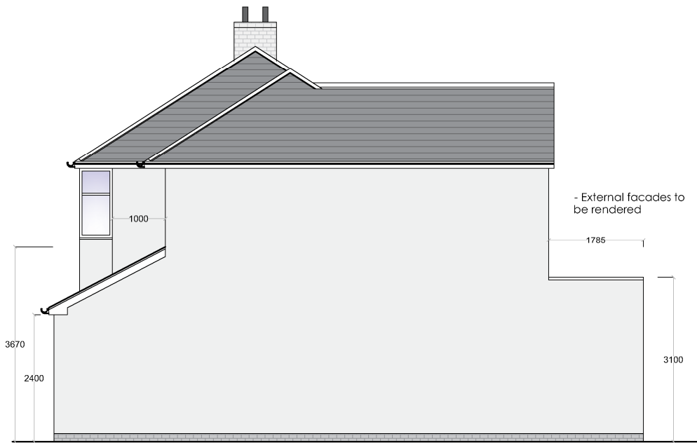
PROPOSED SIDE ELEVATION (Scale 1:100) SCALE BAR - (mm) 500 1000 2000
