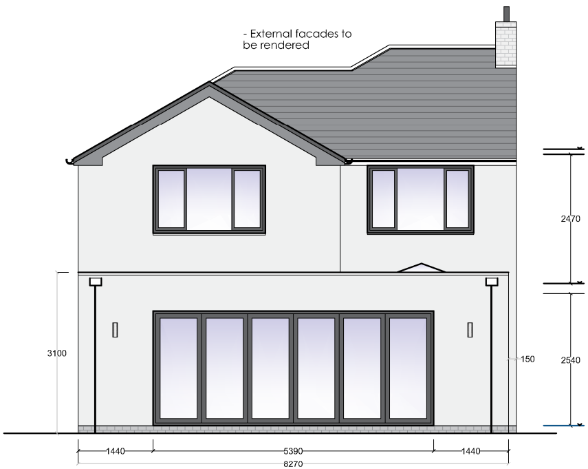
PROPOSED REAR ELEVATION (Scale 1:100) SCALE BAR - (mm) 500 1000 2000
