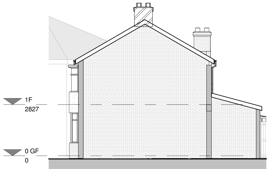
SIDE ELEVATION II
