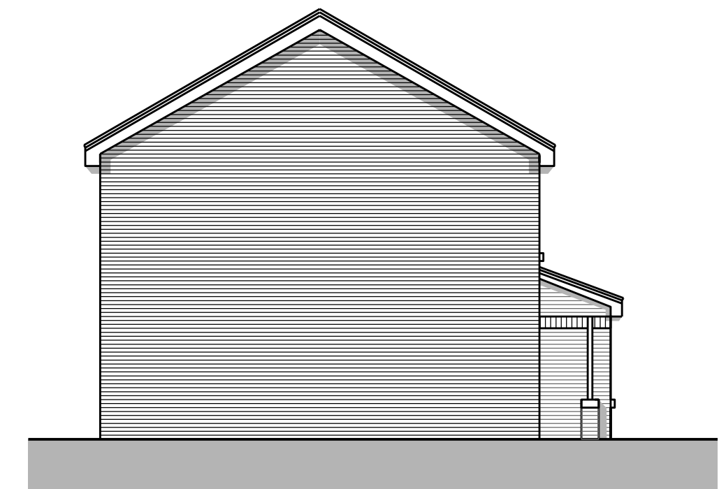
North Elevation(C)
