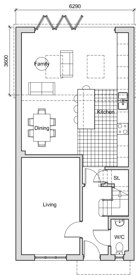
Proposed G/F Plan 1:100
