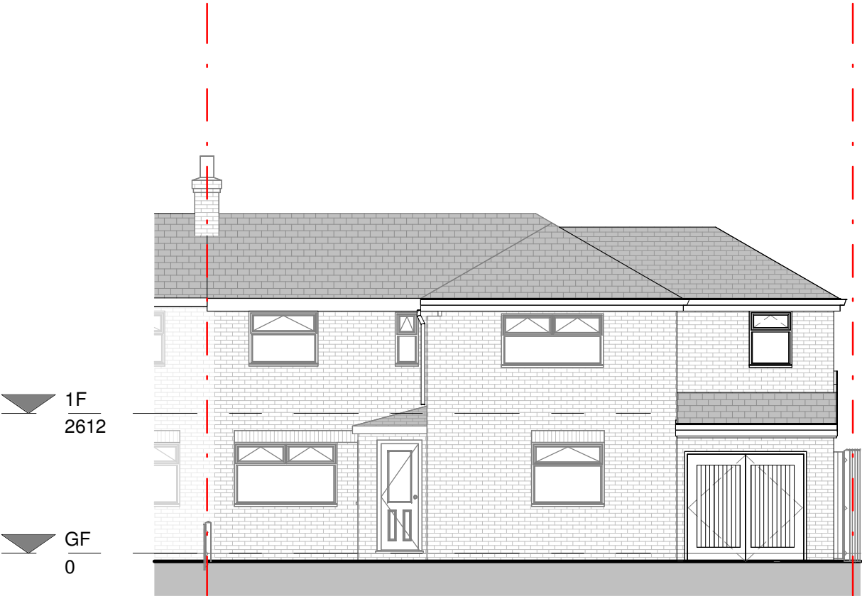
FRONT ELEVATION
