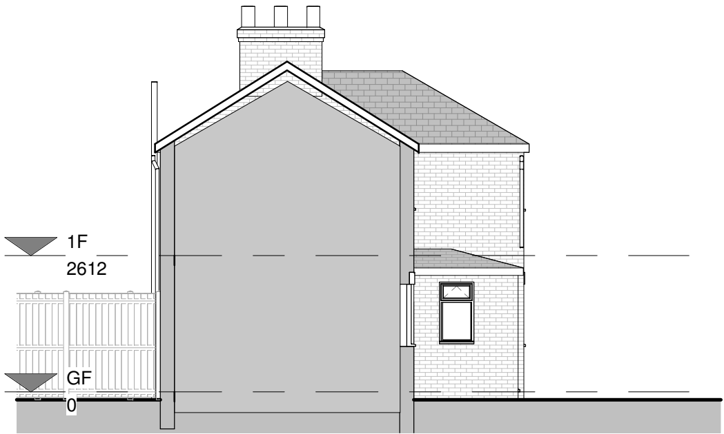
SIDE ELEVATION II
