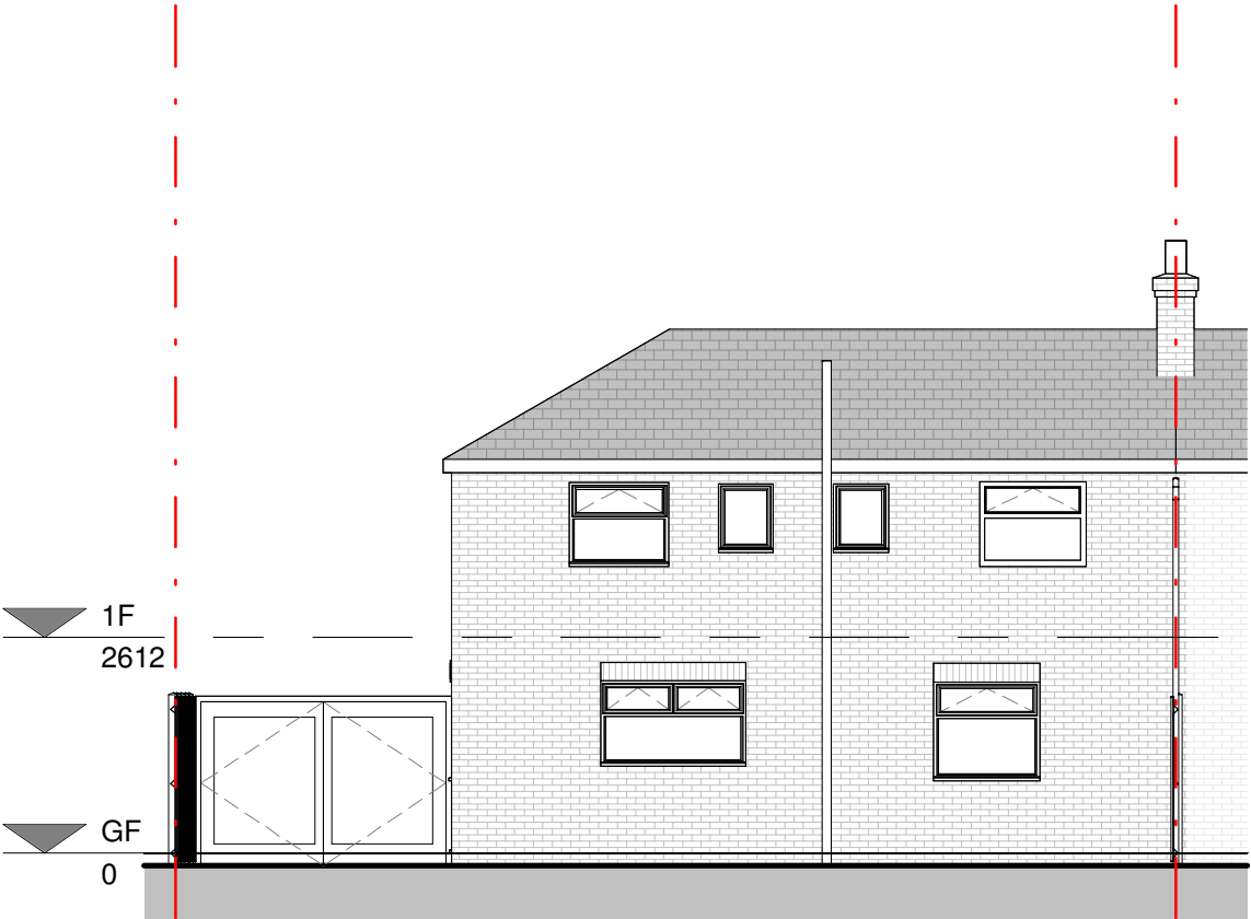
REAR ELEVATION
