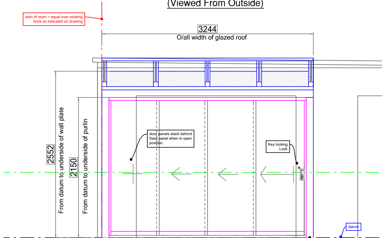
Front Elevation (Viewed From Outside)
