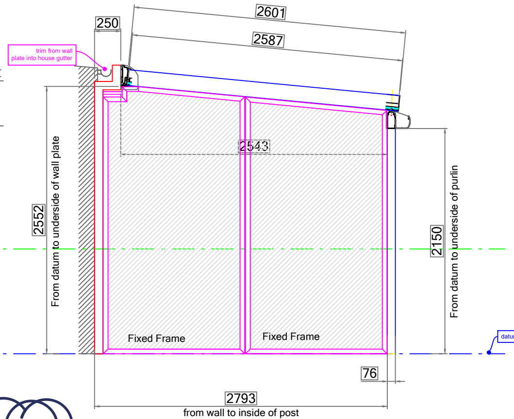
LHS Elevation (Viewed From Outside)
