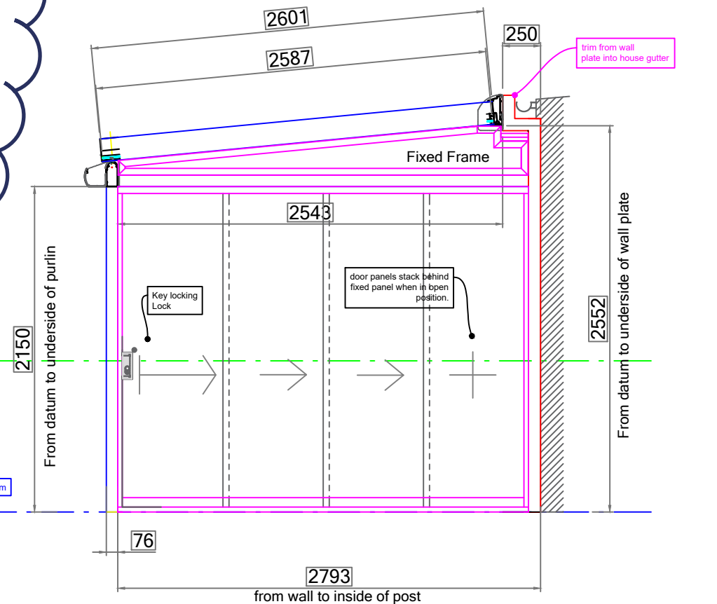
RHS Elevation (Viewed From Outside)
