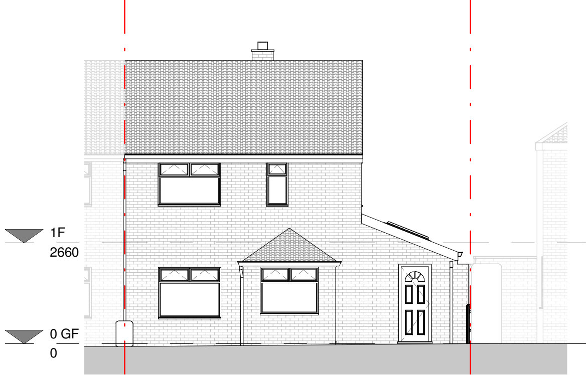
FRONT ELEVATION
