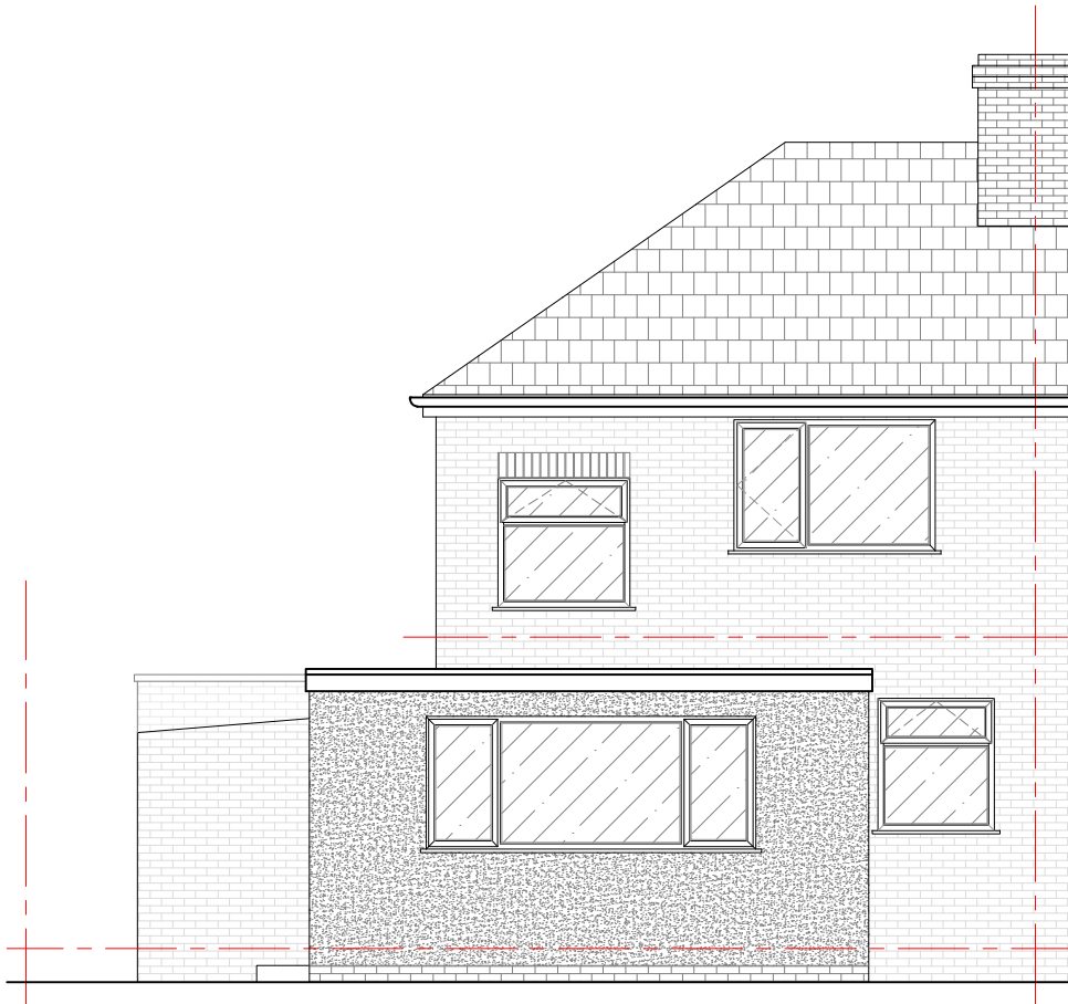
Existing Rear Elevation (Scale - 1:75)
