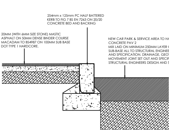
FLAT KERB DETAILS - DETAIL FK - 1:10 (TARMAC PAVING TO CAR PARK TARMAC)
