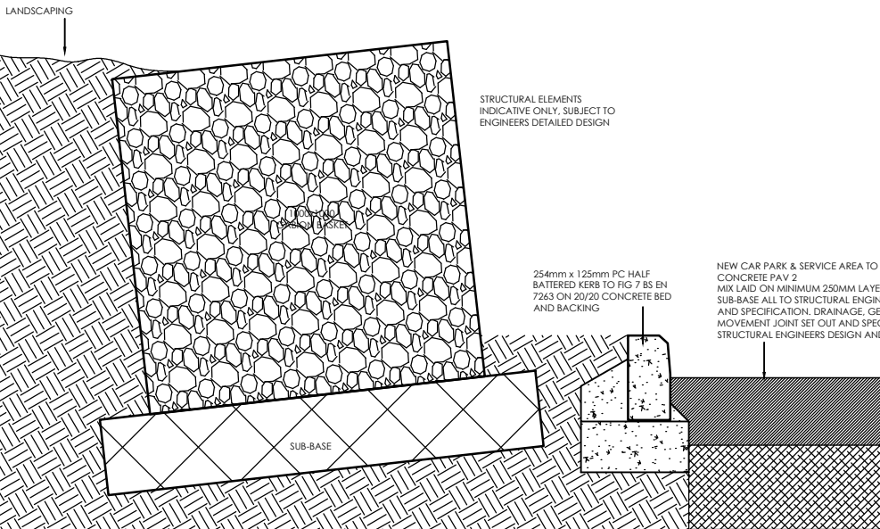
ROAD KERB DETAILS - DETAIL RK - 1:10 CAR PARK TARMAC TO LANDSCAPING
