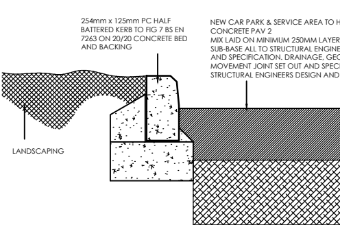
ROAD KERB DETAILS - DETAIL RK - 1:10 (CAR PARK TARMAC TO LANDSCAPING)
