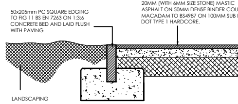
PIN KERB DETAILS - DETAIL PK - 1:10 (TARMAC PAVING TO LANDSCAPING)
