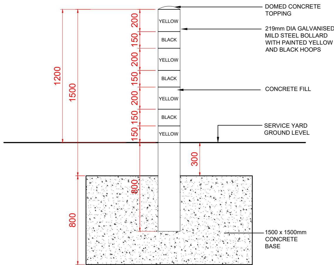
Heavy Duty Bollard Detail - 1:20
