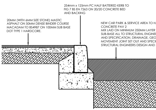
ROAD KERB DETAILS - DETAIL RK - 1:10 (TARMAC PAVING TO CAR PARK TARMAC)
