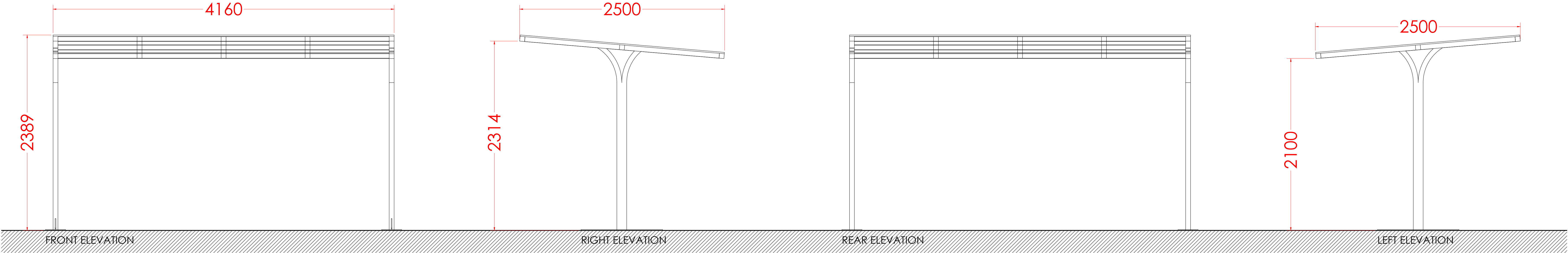
Cycle Shelter Elevations - 1:20
