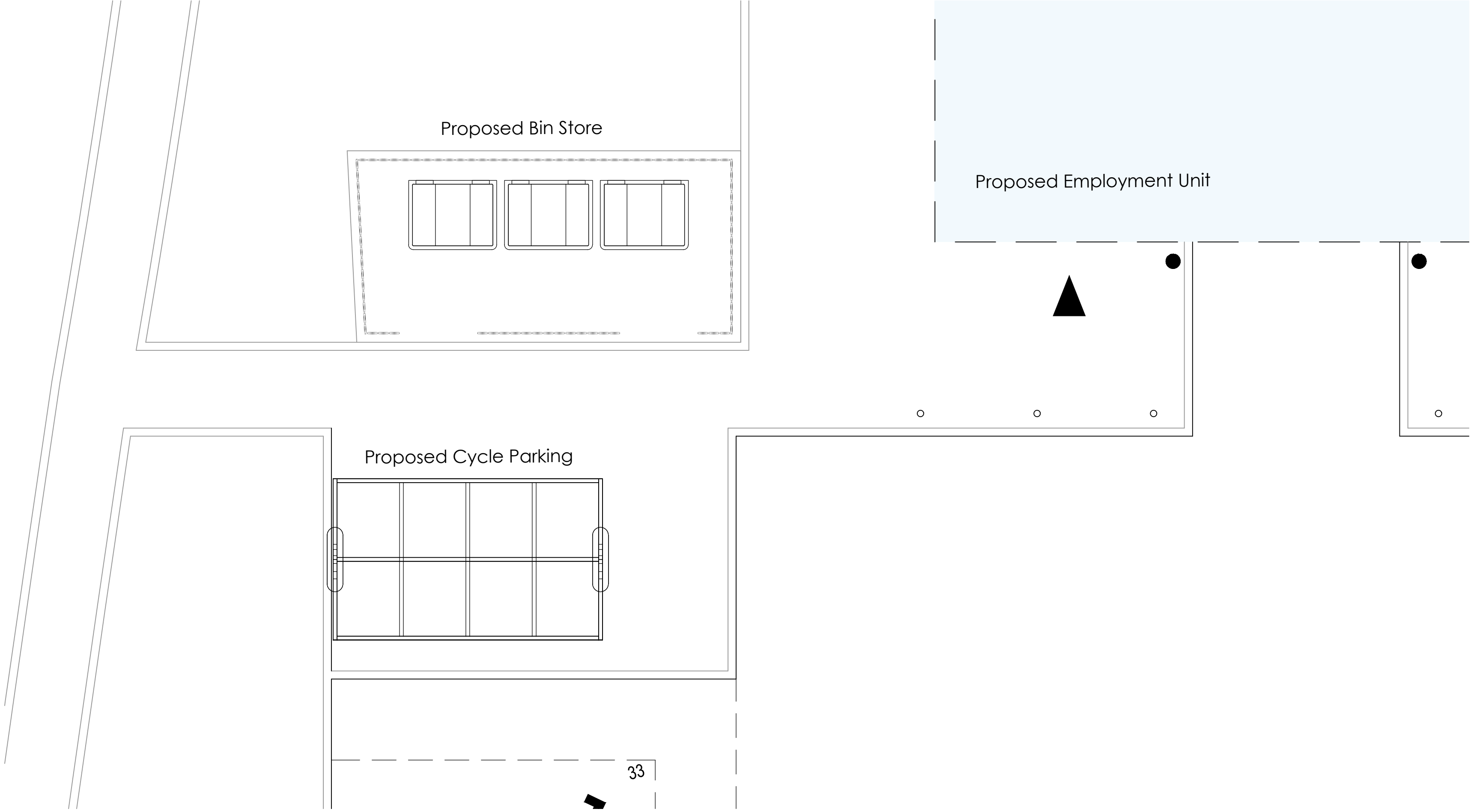
South Cycle Shelter - 1:50
