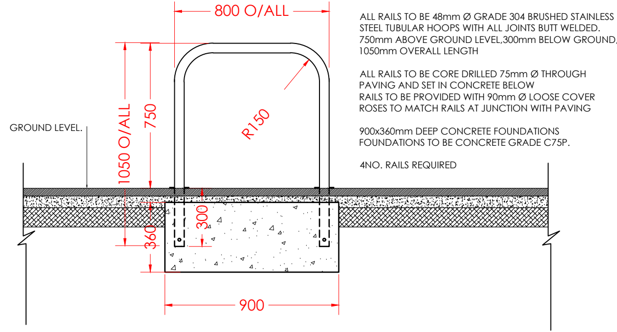
Stainless Steel Cycle Hoop - 1:20
