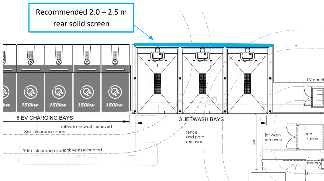
Figure 1 – Figure showing recommended 2.0 – 2.5 m acoustic barrier about rear of proposed jet wash bays.
