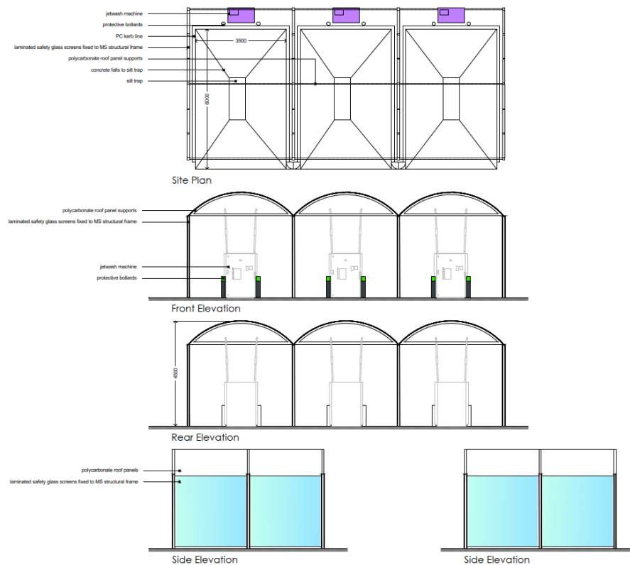
Figure C3 – Proposed jetwash bay design plans.
