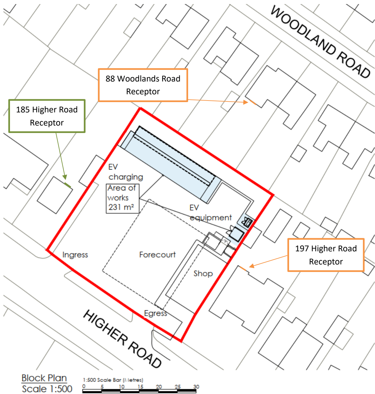
Figure B2 – Location Block Plan, with closest receptors annotated.
