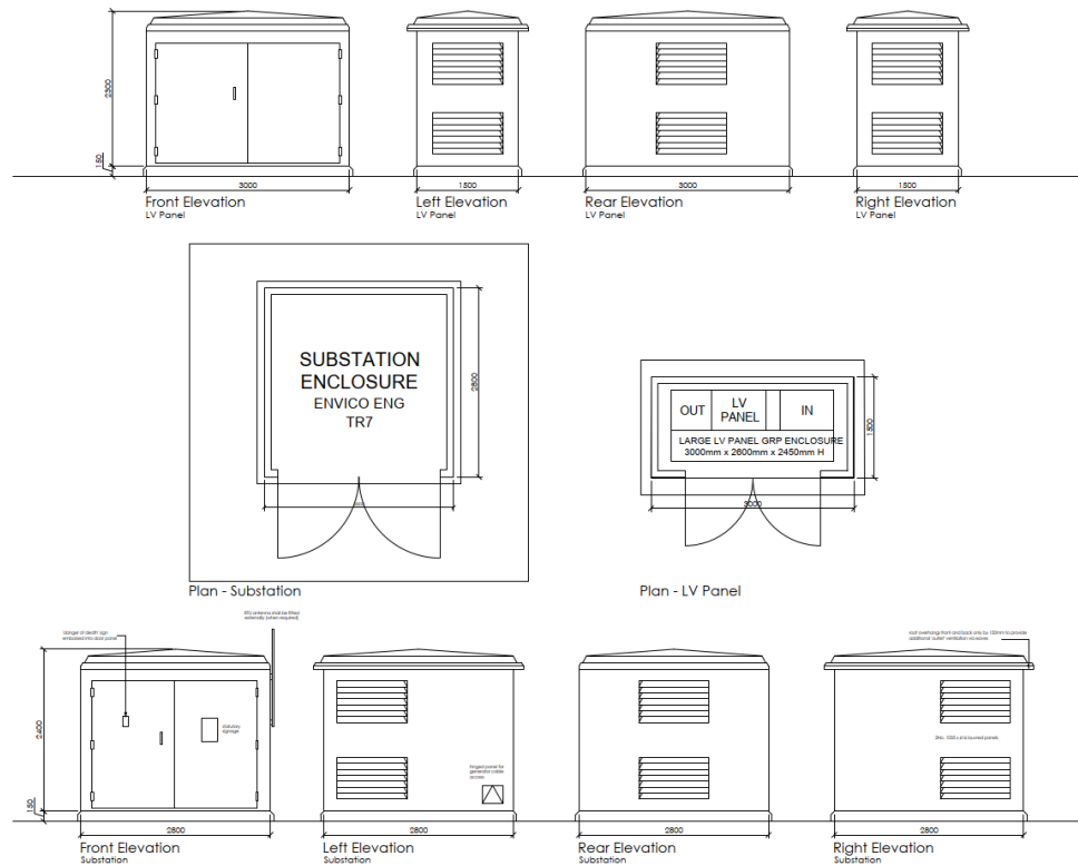
Figure C2 – Proposed substation enclosure (Envico ENG TR7).
