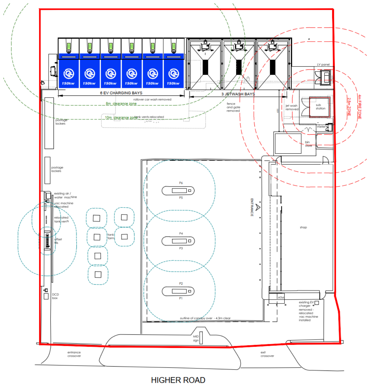
Figure C1 – Proposed development site plan.
