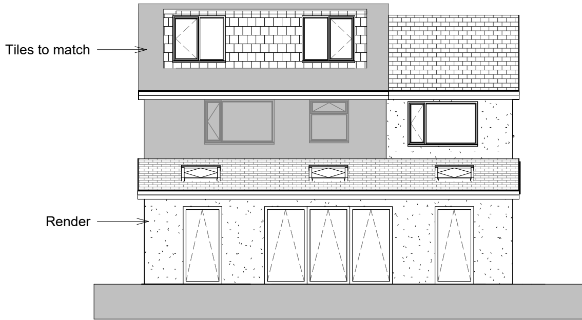
Rear Elevation
