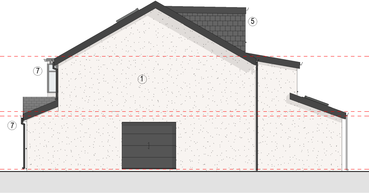
Proposed Side Elevation (No. 42) 1 : 100
