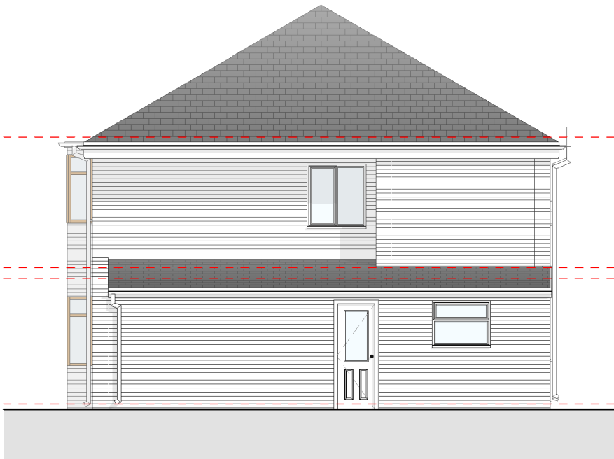
Existing Side Elevation (No. 42) 1 : 100
