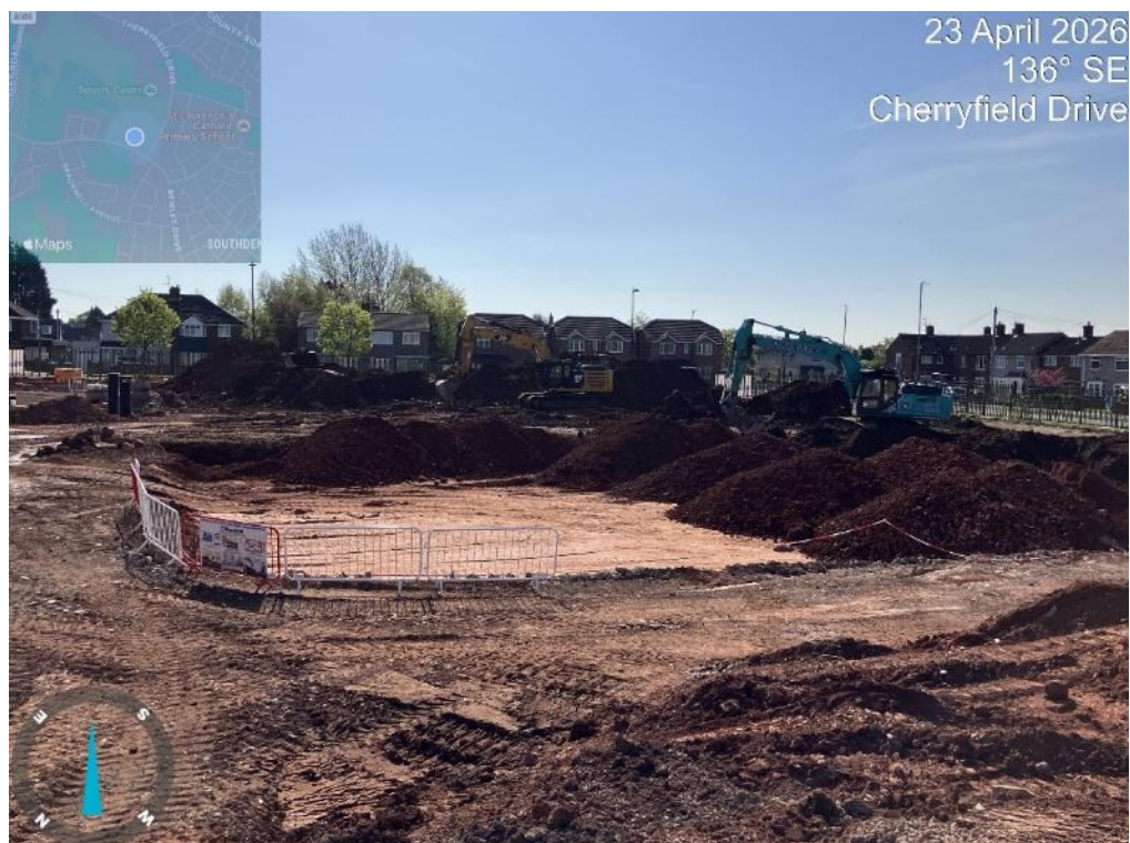
Plate 18 Upfill with Site-Won Granular / Non-Heave Impacted Cohesive Materials
