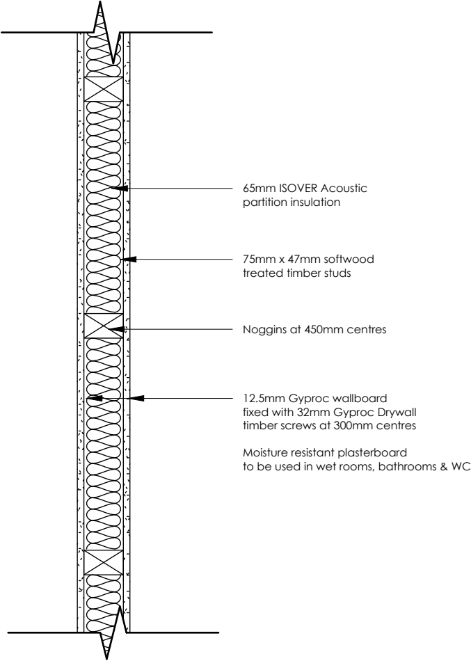
GBA-IW2 Internal Timber stud wall Insulated habitable room and wet rooms
