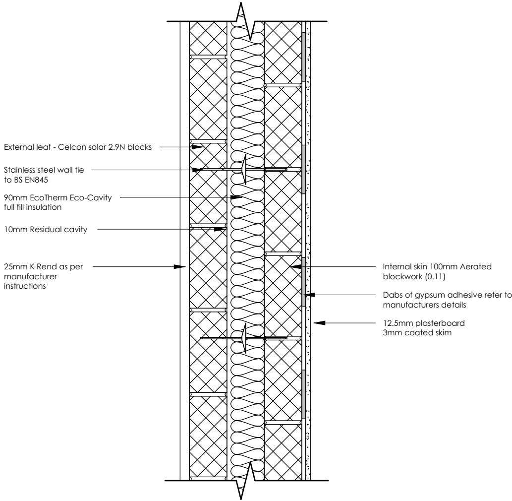
GBA-EW2 External block cavity wall render finish External wall to meet minimum U-Value 0.18W/m²K
