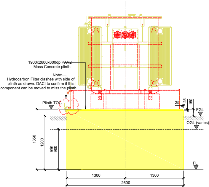
Section 02
