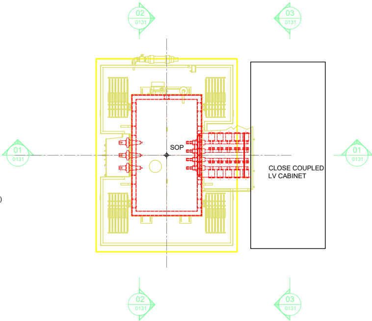
Foundation Plan
