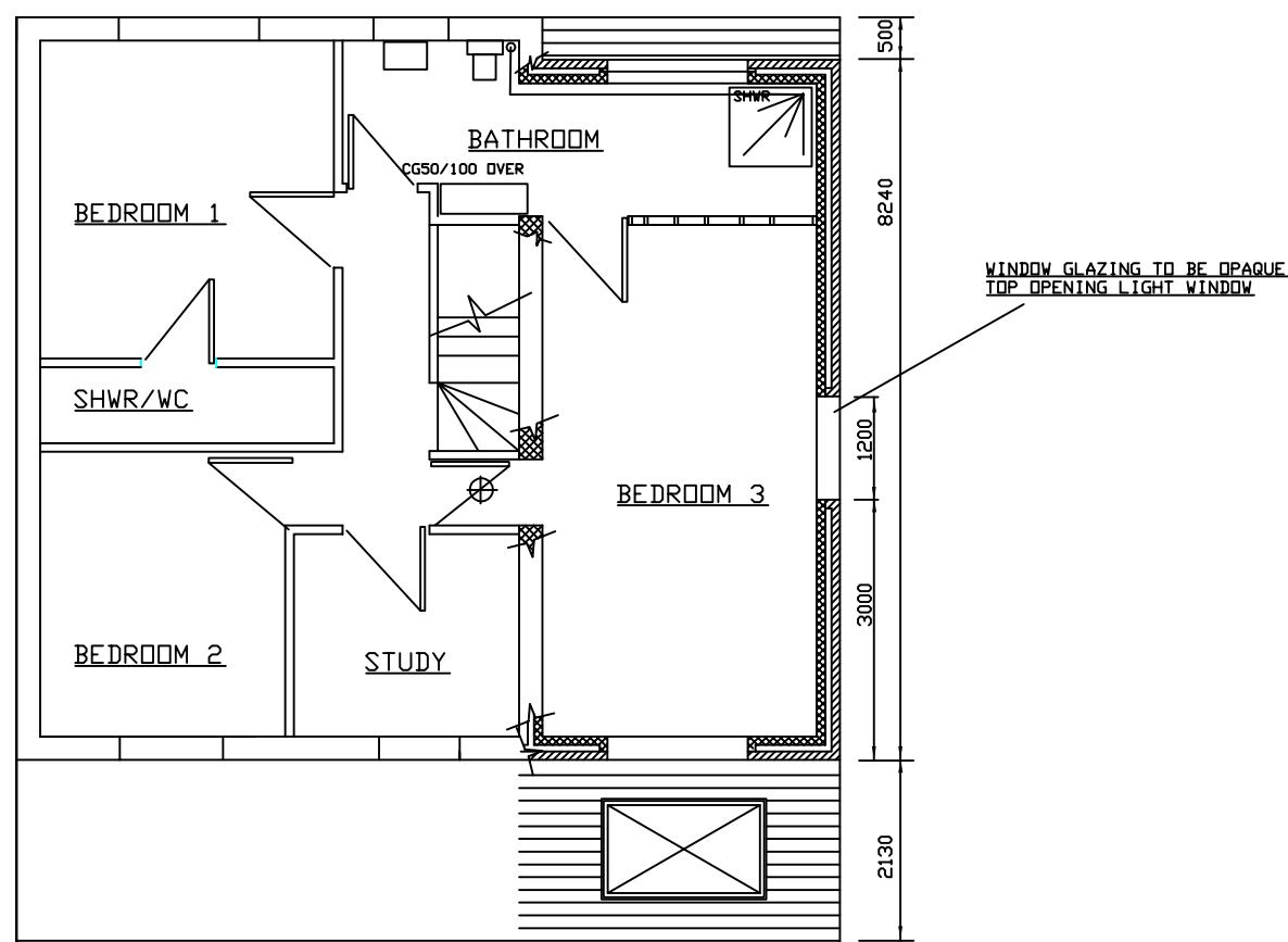
PLAN ON PROPOSED FIRST FLOOR WITH FLOOR STRUCTURE REMOVED
