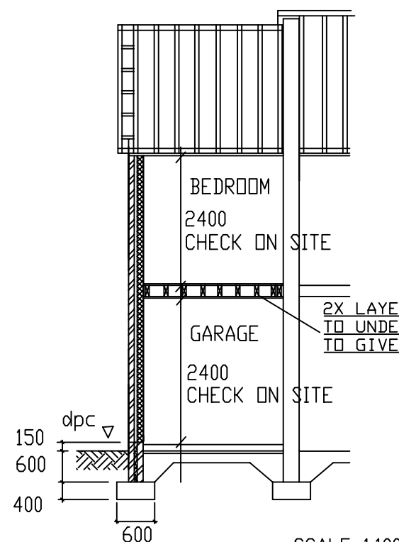
SCALE 1:100 TYPICAL SECTION THRO ON EXTENSION
