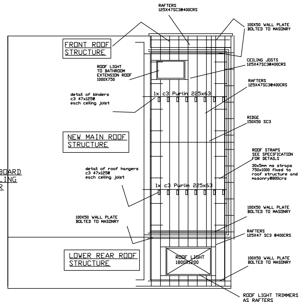
PLAN ON ROOF STRUCTURES SCALE 1:100
