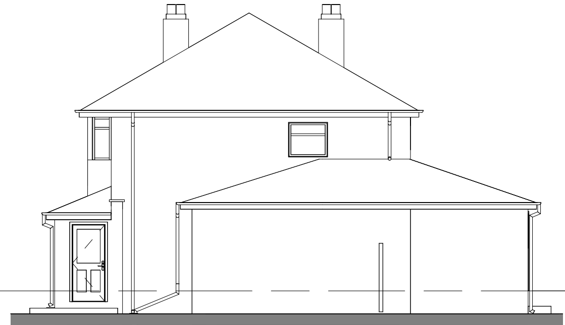
4 Side Elevation 2 as Existing 1 : 100
