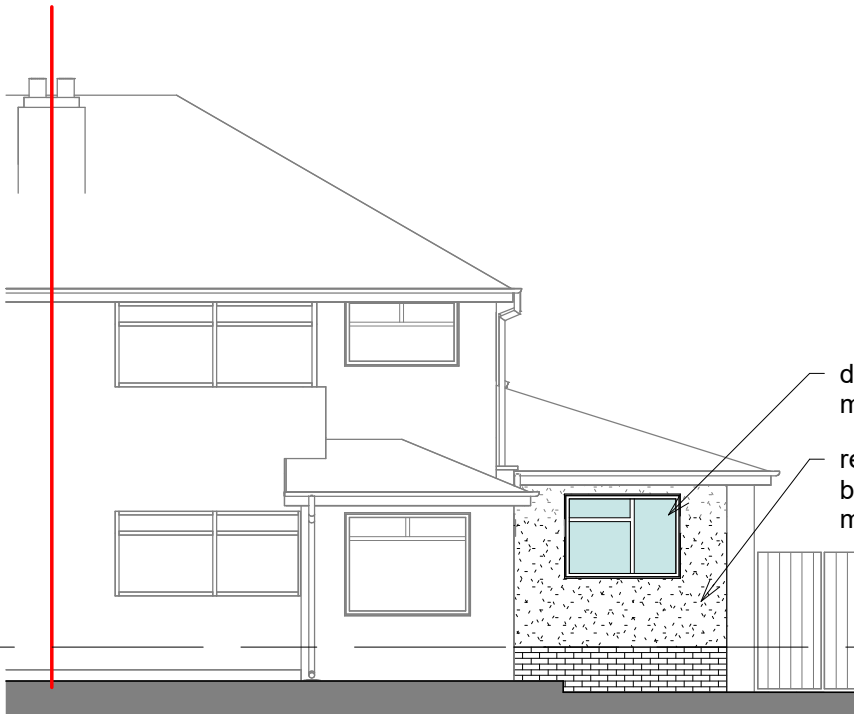
1 Front Elevation as Proposed 1 : 100
