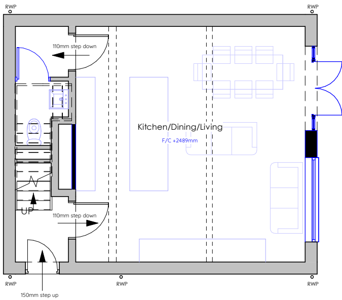
00 Ground Floor - Proposed
