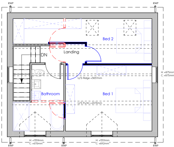
01 First Floor - Proposed
