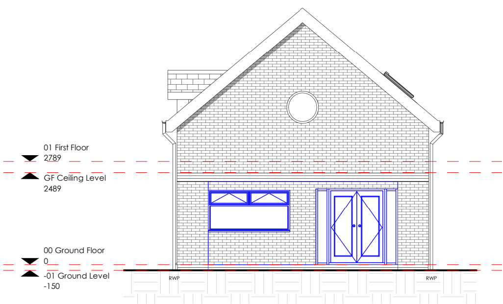
Elevation 1 - Proposed
