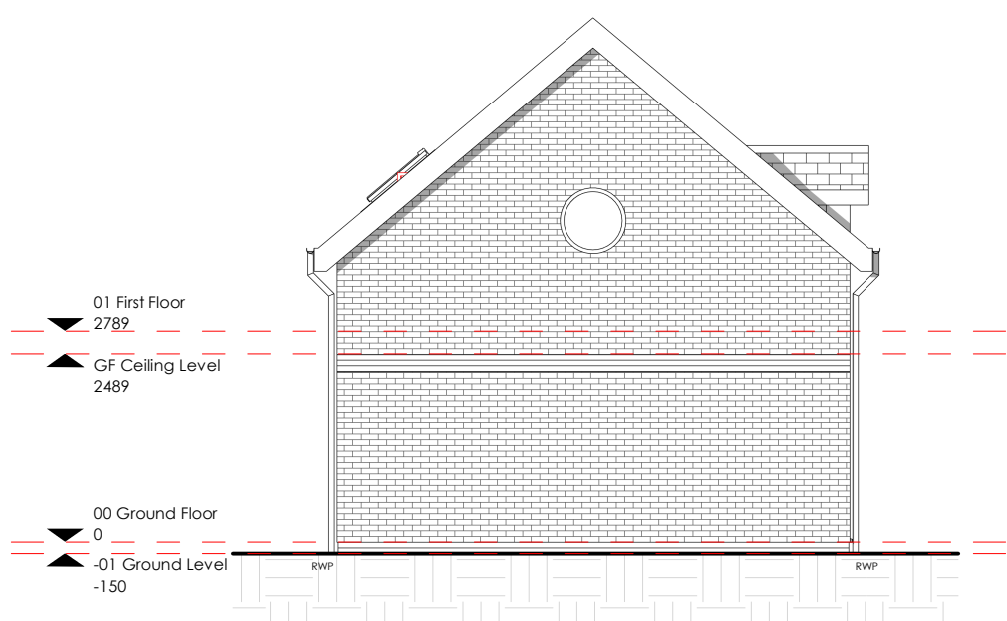
Elevation 3 - Proposed
