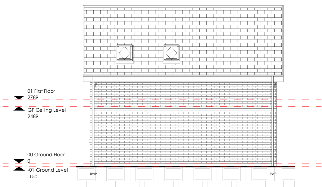
Elevation 4 - Proposed
