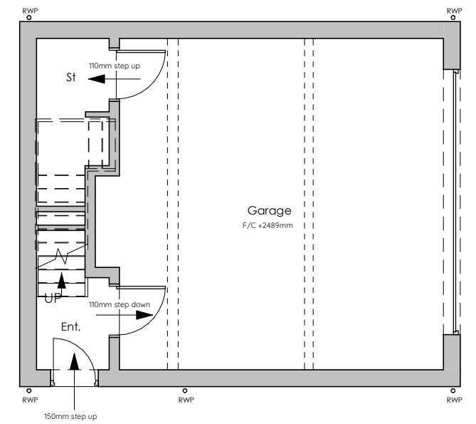
00 Ground Floor
