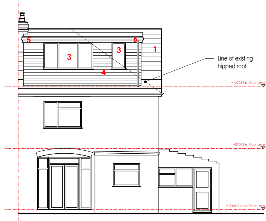
Rear Elevation
