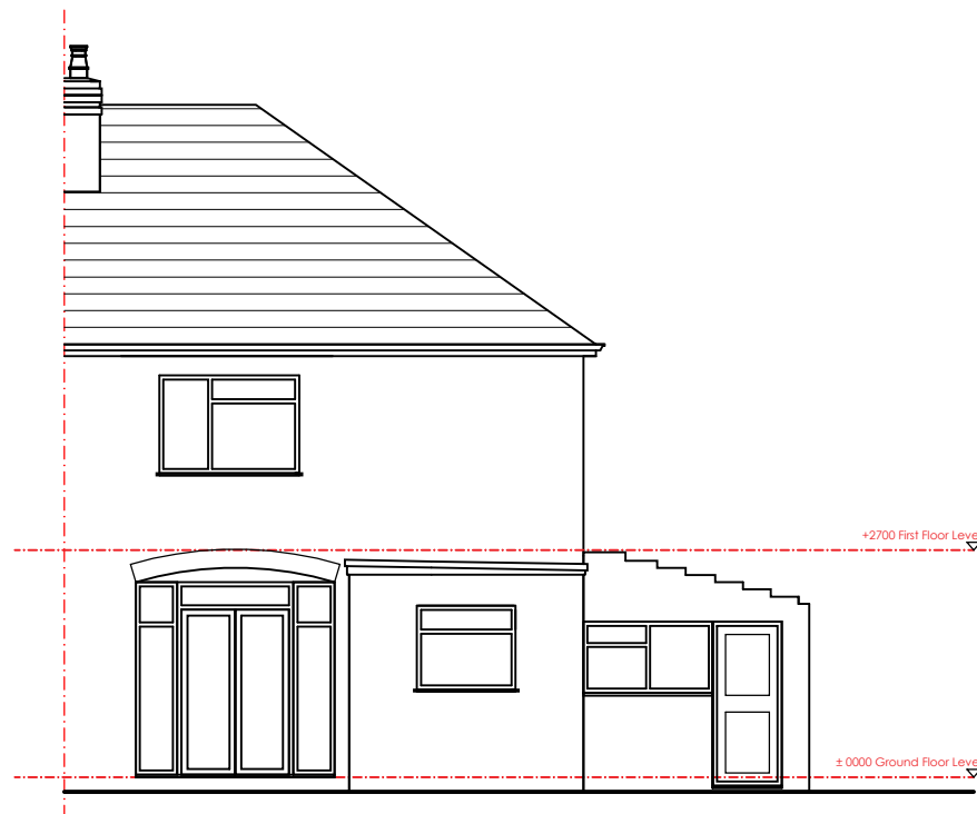
Rear Elevation
