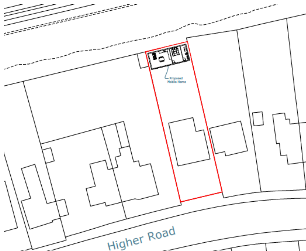
Figure 1: Extract from proposed block plan, showing the intended location of the proposed mobile home.
