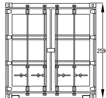
Front end
