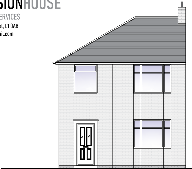
EXISTING FRONT ELEVATION (Scale 1:100) SCALE BAR - (mm) 500 1000 2000
