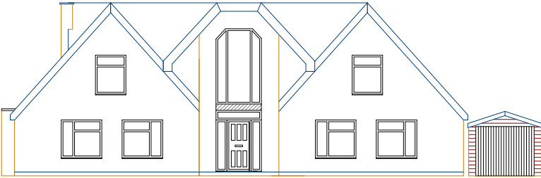
PROPOSED FRONT ELEVATION
