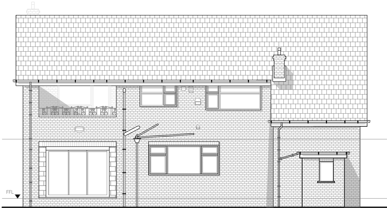
Existing Rear Elevation Scale 1:100@A3
