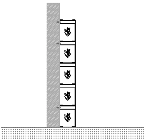
Fixing Specification
