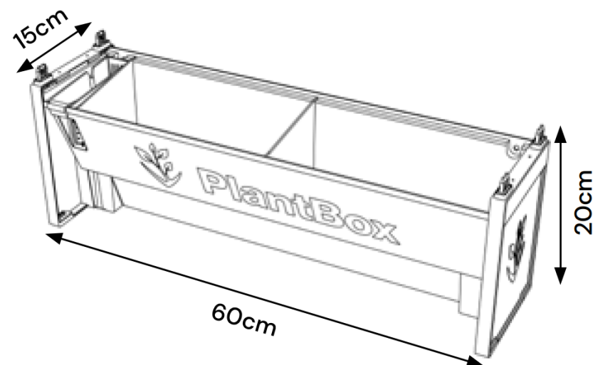
Unit Dimensions
