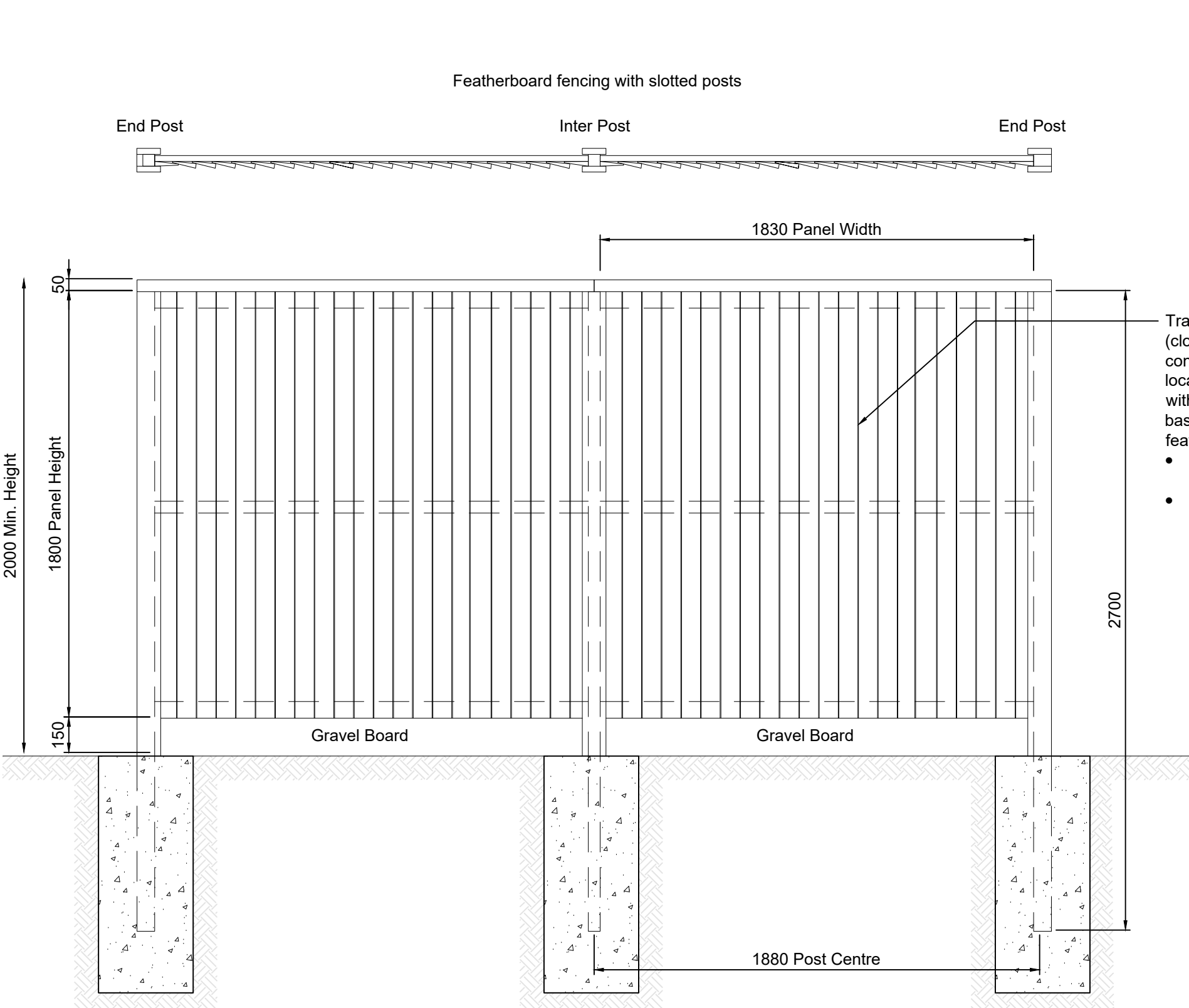
Timber Fence Details Scale 1:20
