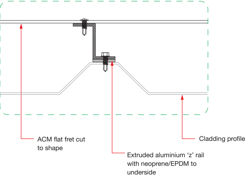
FIXING METHOD
