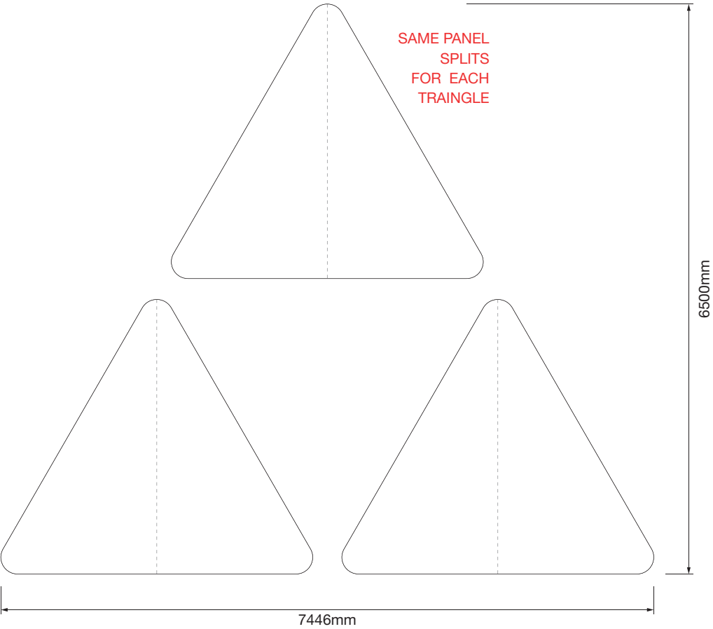
PLAN VIEW
