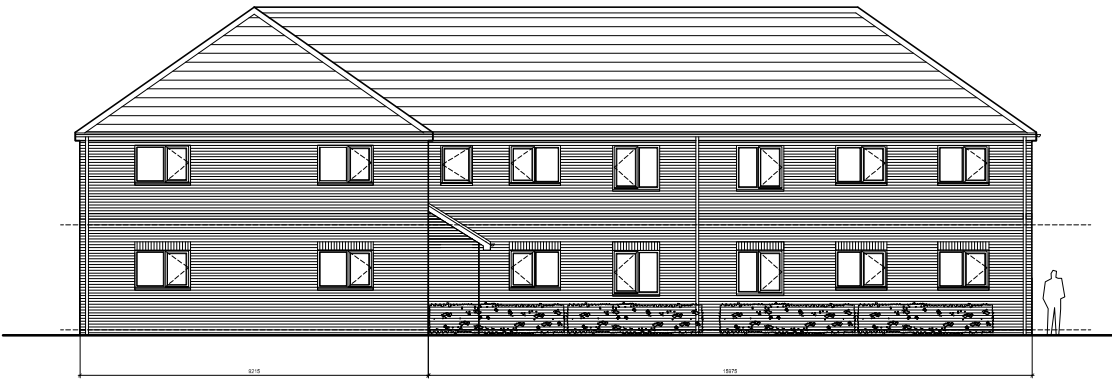
East Elevation (facing park)
