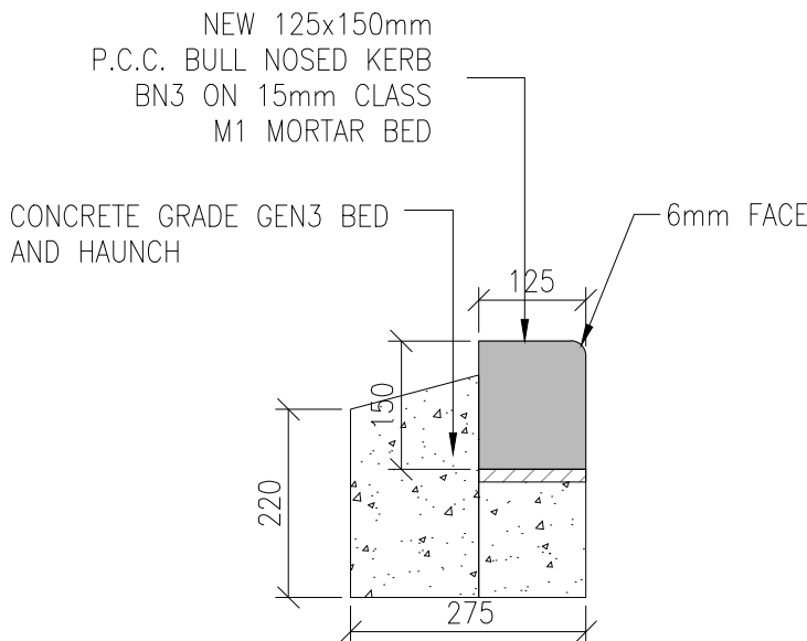
BN3 BULL NOSE DROP KERB DETAIL SCALE: 1:10 @ A1
