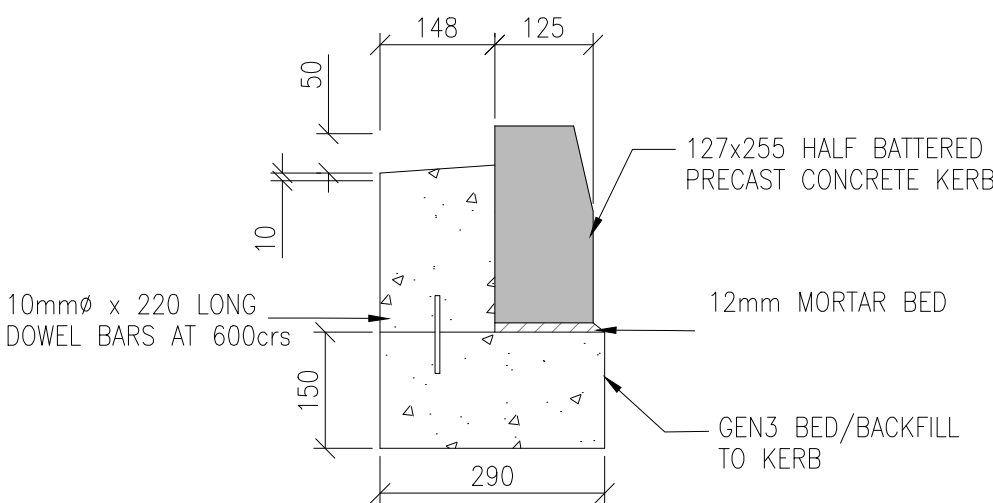
HALF BATTERED 2 & TRANSITION BENNING DETAIL SCALE: 1:10 @ A1
