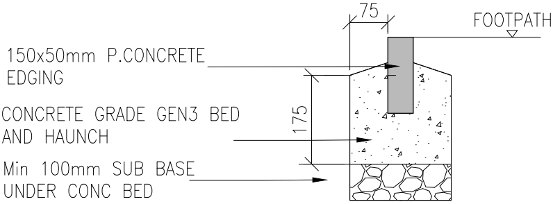
FOOTPATH EDGING DETAIL SCALE: 1:10 @ A1
