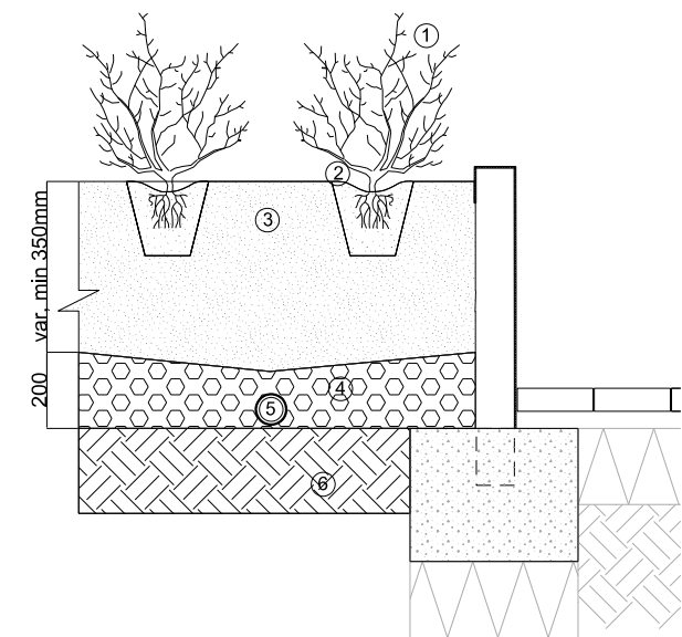
PP01 TYPICAL PLANTING IN PLANTERS SECTION
