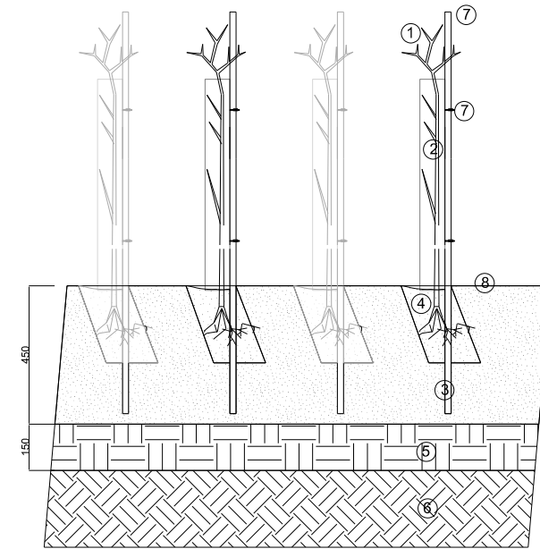
HP01 TYPICAL HEDGE PLANTING SECTION
