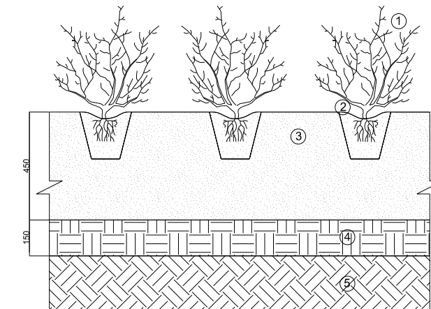
SP01 TYPICAL SHRUB, PERENNIAL AND ORNAMENTAL GRASS PLANTING SECTION
