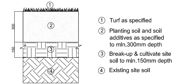
GP01 TYPICAL GRASS PLANTING SECTION
