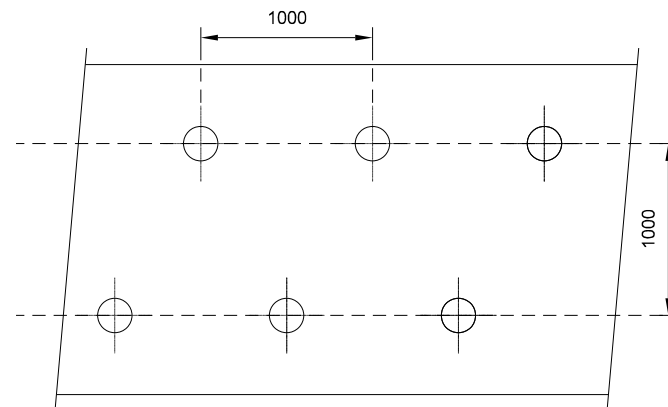
HP02 TYPICAL HEDGE PLANTING PLAN
