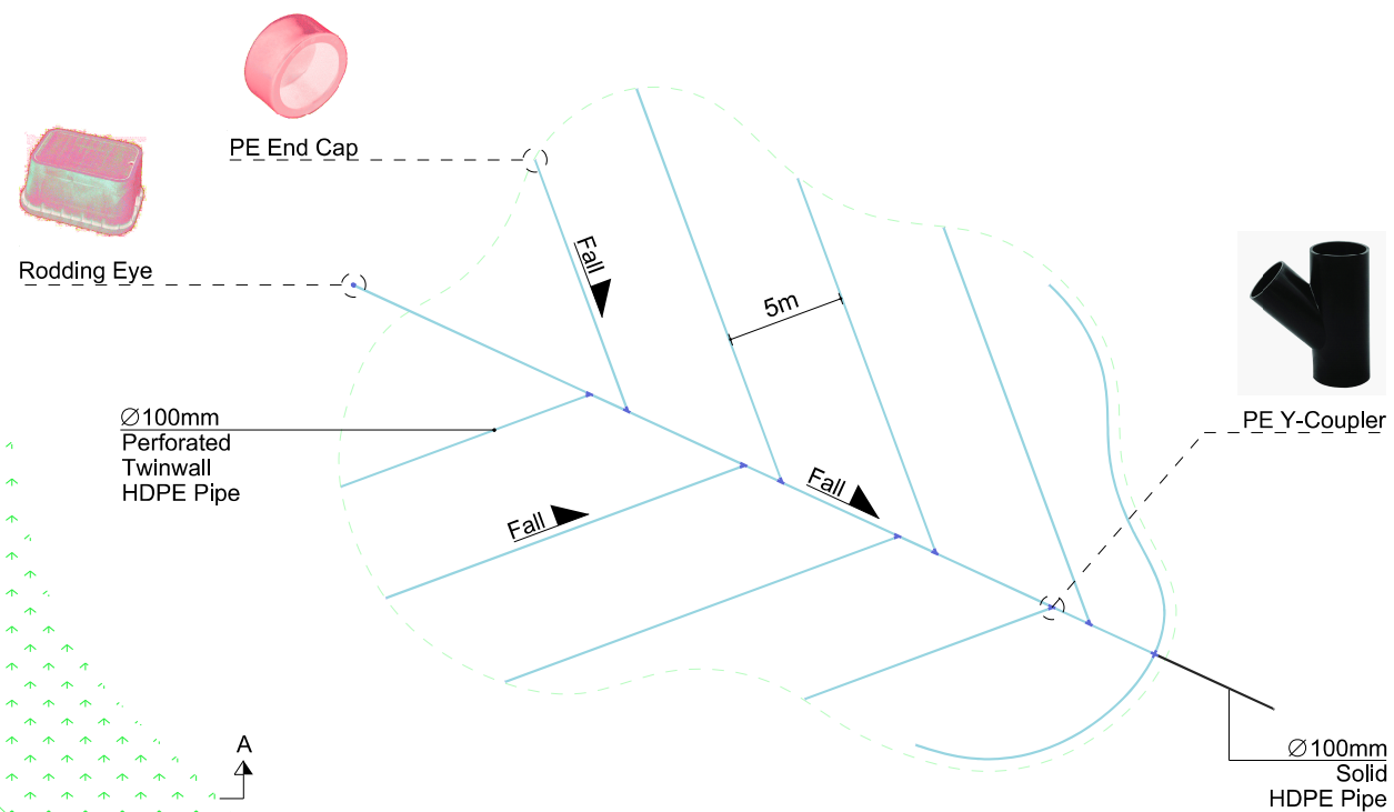
GD01 TYPICAL GREEN DRAINAGE LAYOUT
