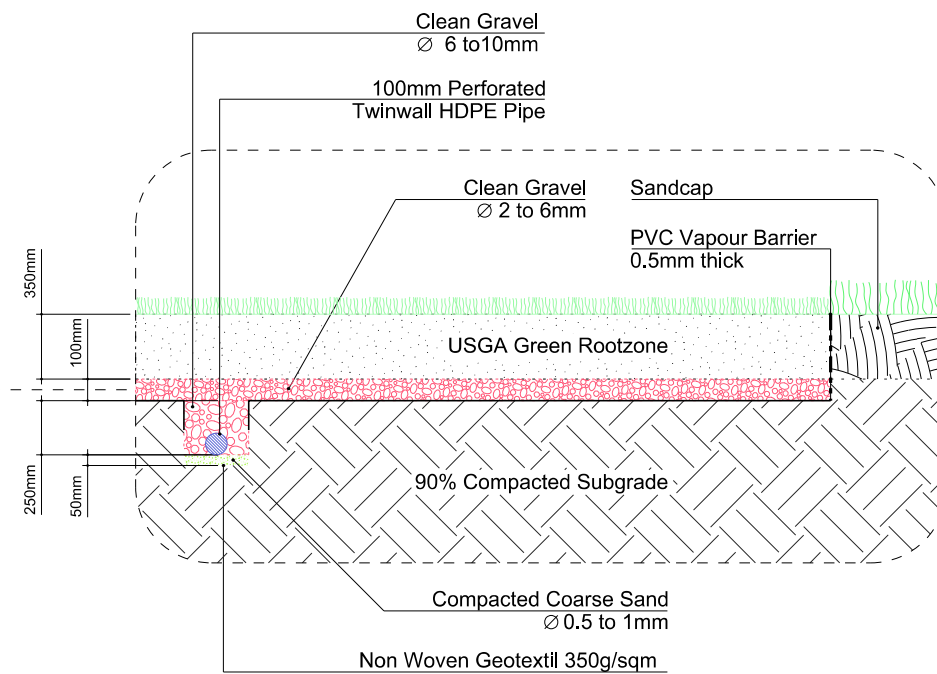
GD02 TYPICAL GREEN DRAINAGE DETAIL
