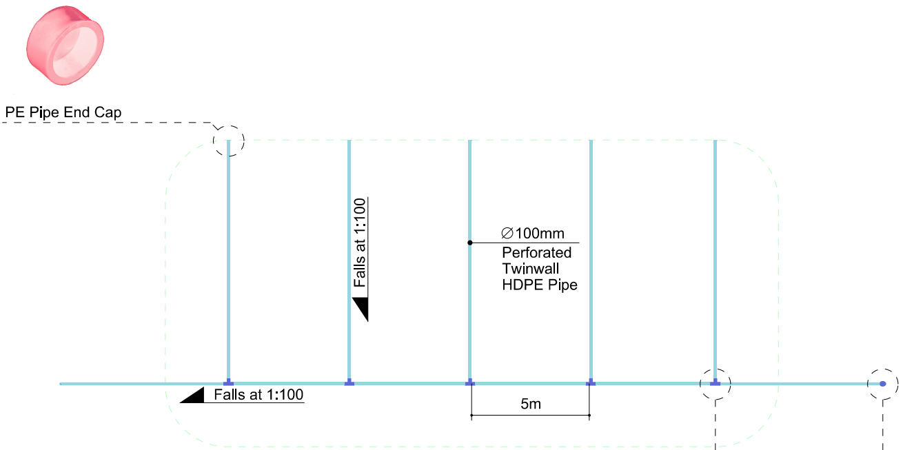
TD01 TYPICAL TEE DRAINAGE LAYOUT
