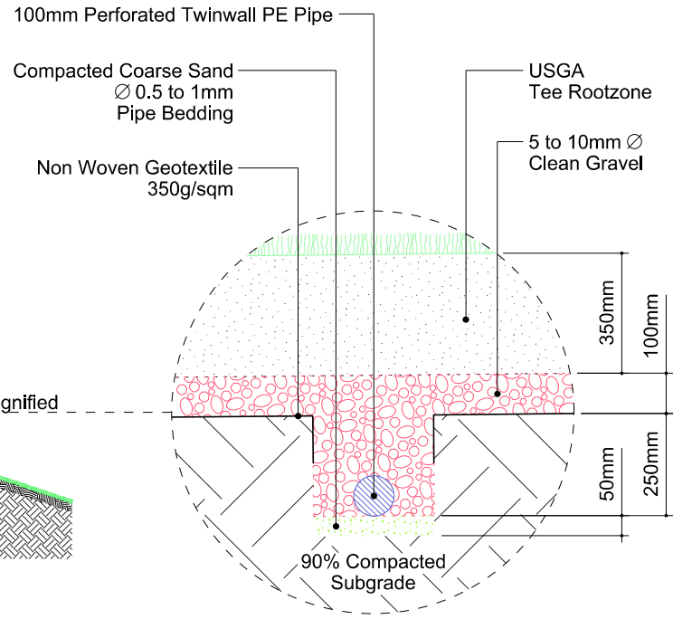
TD02 TEE DRAINAGE DETAIL
