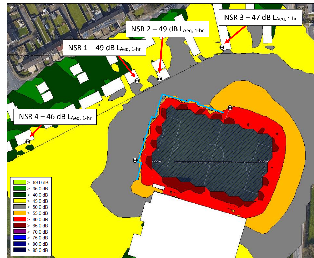
Figure 5: AGP and crowd speaking with raised voices calculated L_{Aeq,1hr} noise contours at 1.5 m height
