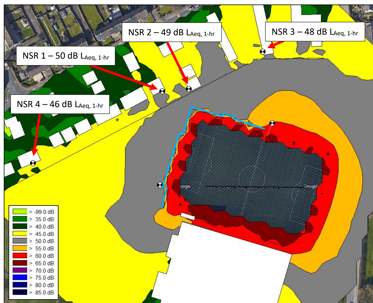
Figure 4: AGP and crowd cheering calculated L_{Aeq,1hr} noise contours at 1.5 m height
