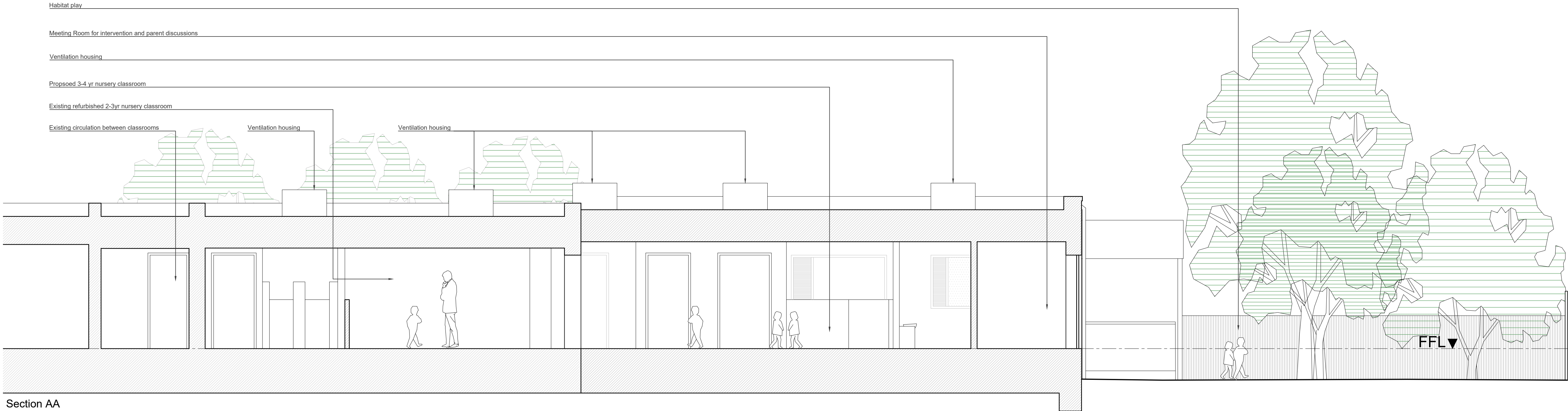
Section AA
