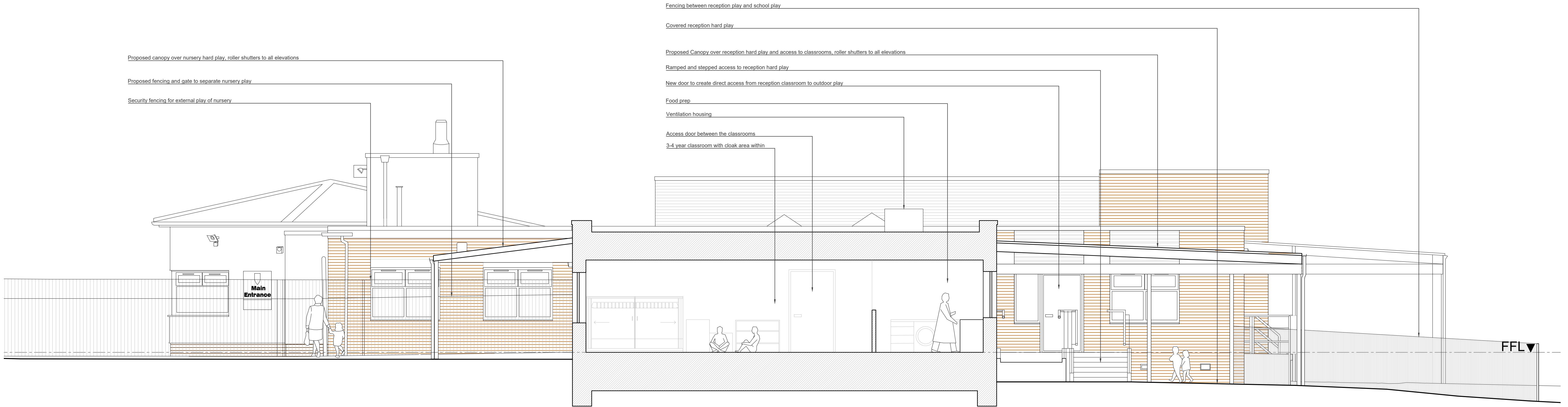
Section BB
