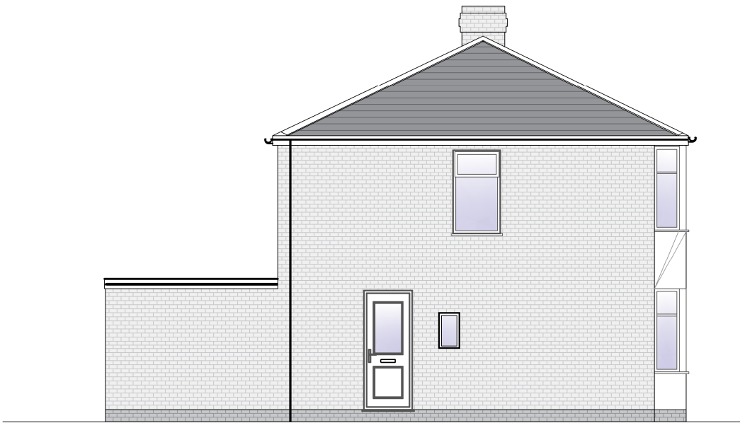
EXISTING SIDE ELEVATION (Scale 1:100) SCALE BAR - (mm) 500 1000 2000
