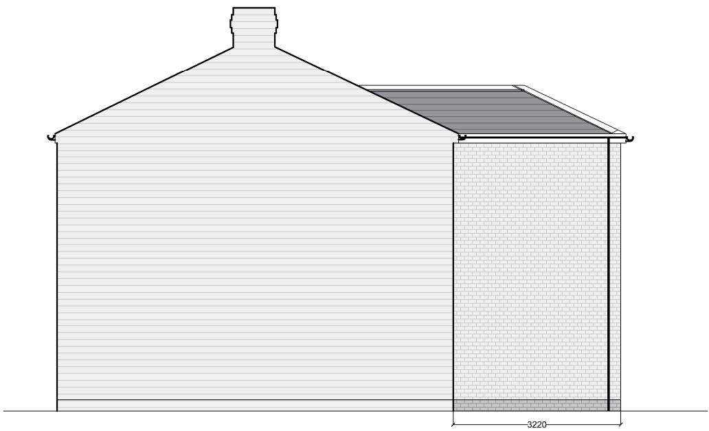
PROPOSED SIDE ELEVATION (Scale 1:100) SCALE BAR - (mm) 2000 1000 500
