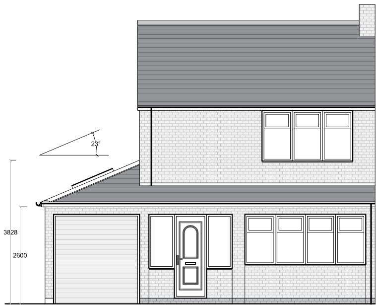
PROPOSED FRONT ELEVATION (Scale 1:100) SCALE BAR - (mm) 500 1000 2000
