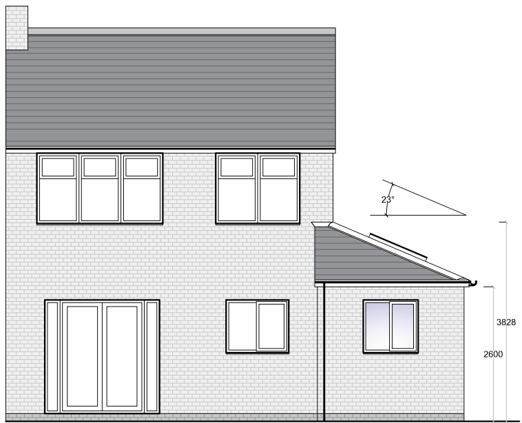
PROPOSED REAR ELEVATION (Scale 1:100) SCALE BAR - (mm) 500 1000 2000
