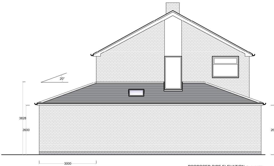
PROPOSED SIDE ELEVATION (Scale 1:100) SCALE BAR - (mm) 2000 1000 500
