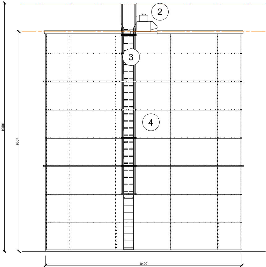
PROPOSED ELEVATION
