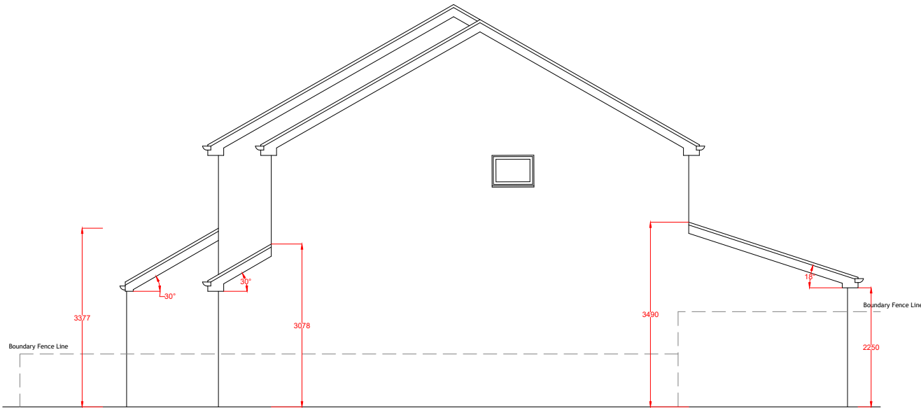
Proposed North Side Elevation 1:100
