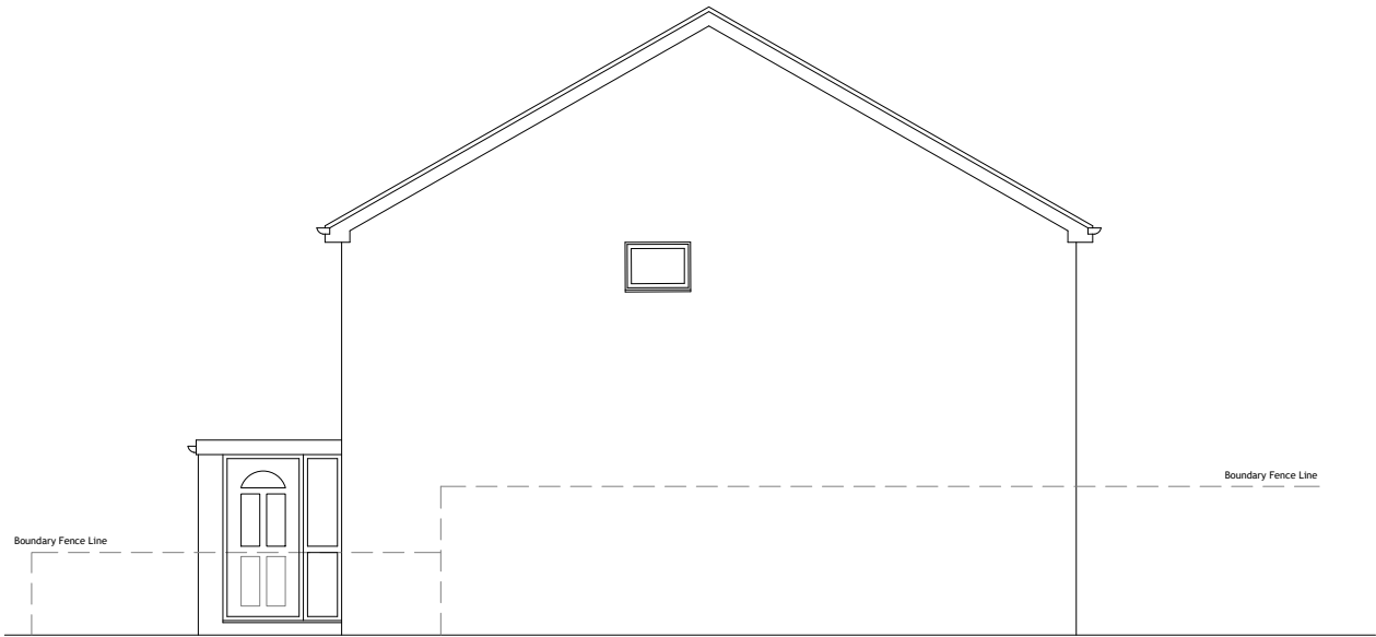
Existing North Side Elevation 1:100
