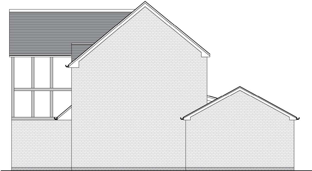
EXISTING SIDE ELEVATION (Scale 1:100) SCALE BAR - (mm) 0 500 1000 2000
