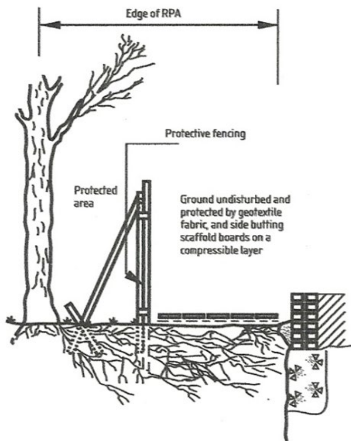
Figure 2. Ground protection with scaffolding boards within the RPA (taken from BS5837:2005)
